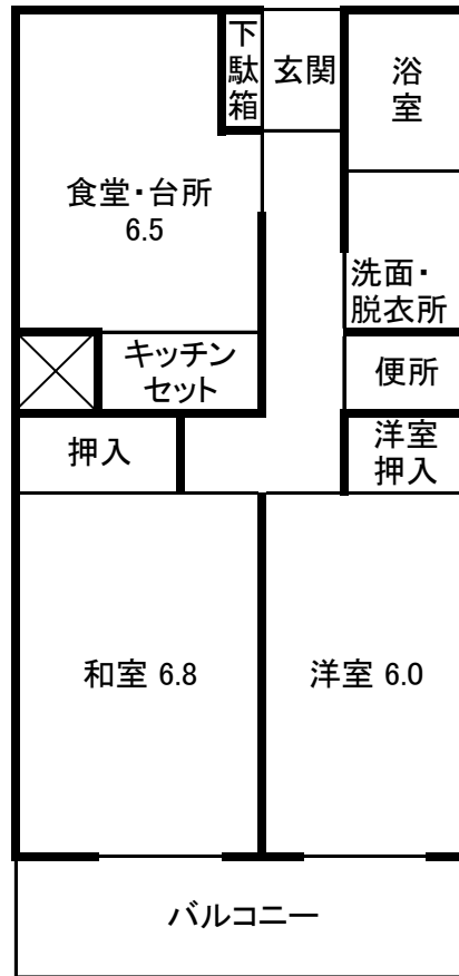
2DK 54.1㎡
