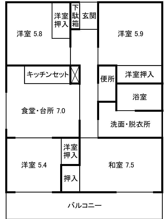
4DK 78.6㎡
